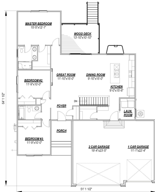
MAIN LEVEL
