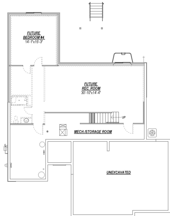
LOWER LEVEL
